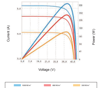
I-V Curves
